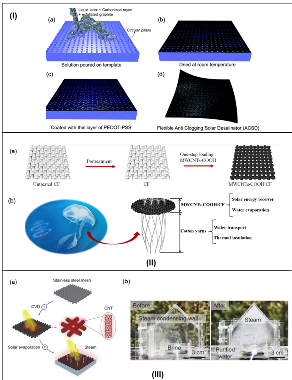
Fig. 10 Carbon-based SIWE devices. (I) Solar desalination via flexible graphite film (a–c) schematic representation of the fabrication of the ACSD (anti-clogging solar desalinators). Reproduced with permission. 108 Copyright 2017, Royal Society of Chemistry. (II) MWCNTs-COOH/CF solar evaporator. (a) Preparation, and (b) representation of the inspiration for the designed system. Reproduced with permission. 138 Copyright 2020, Elsevier. (III) Single-layer CNT-based photothermal film. (a) Schematic diagram of the preparation process and evaporation via the prepared film and (b) the practical applications before and after the operation. Reproduced with permission. 140 Copyright 2020, Acta Physico-Chimica Sinica.
