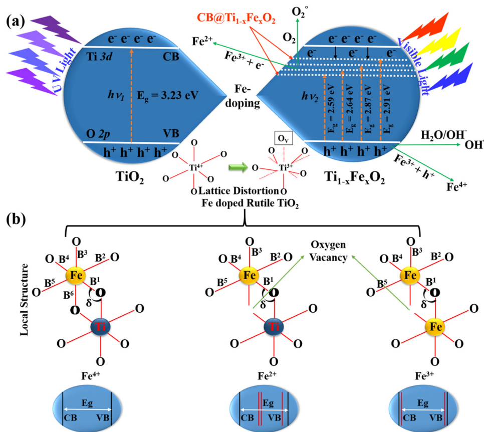
Fig. 1 (a) The process of charge transport involving elevated electrons and VBs of the TiO 2 nanorods with Fe 3+ ions of Ti 1-x Fe x O 2 (x = 0–0.1), and (b) schematics of the local topologies of Fe-dopants in the different Fe 4+ , Fe 2+ , and Fe 3+ doped TiO 2 models respectively. B 1–6 are the bond lengths of Fe–O bonds and \delta is the bond angle between Fe–O–Ti and Fe–O–Fe.
