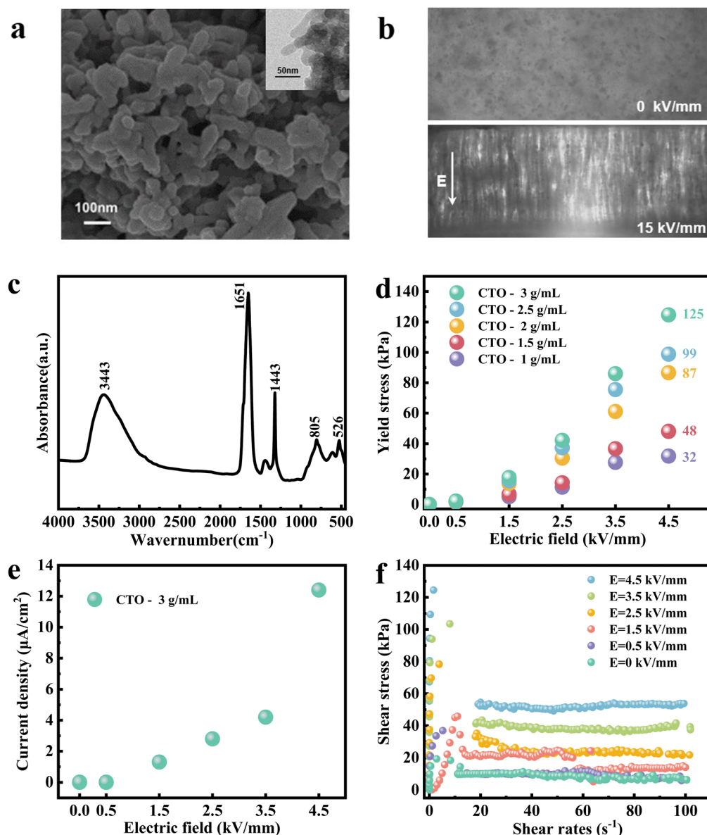
Fig. 2 (a) SEM image and TEM image (inset in a) of the CTO particles. (b) Optical images of the electro-rheological structure without/with the applied electric field. (c) FTIR spectra of the CTO particles. (d) Yield stress of the ER fluids with different concentrations as a function of the applied electric field. (e) Leakage current density of the ER fluid ( 3\text{ g mL}^{-1} ) as a function of the applied electric field. (f) Shear stress of the ER fluid ( 3\text{ g mL}^{-1} ) with the shear rate as a function of the applied electric field.
