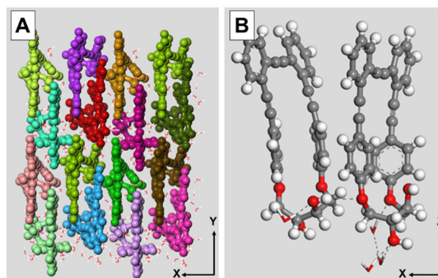
Fig. 3 (A) Top view of a monolayer of ( R,R,M )-1 molecules onto a water surface. XYZ dimension values of the computational box were 24 × 30 × 150 Å 3 . Water molecules are depicted as sticks for clarity. (B) Close detail of ( R,R,M )-1 molecules in the monolayer. Additional ( R,R,M )-1 and water molecules are omitted for clarity. The formation of intermolecular H-bonds between neighbour ( R,R,M )-1 molecules and H-bonds with water is displayed as a dashed black line, left and right, respectively.
