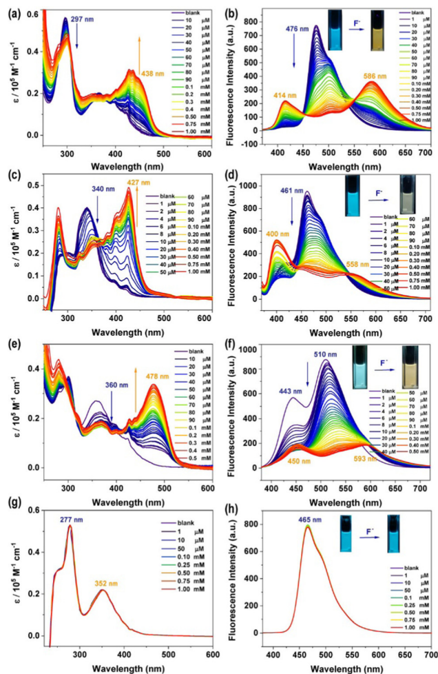
Fig. 3 Spectral changes in the UV/vis absorption (left) and fluorescence (right) after the addition of TBAF. (a) and (b) 3a , \lambda_{\text{ex}} = 365 \text{ nm} , [ 3a ] = 10 \mu\text{M} ; (c) and (d) 3b , \lambda_{\text{ex}} = 365 \text{ nm} , [ 3b ] = 10 \mu\text{M} ; 3c , \lambda_{\text{ex}} = 365 \text{ nm} , [ 3c ] = 10 \mu\text{M} ; 3d , \lambda_{\text{ex}} = 365 \text{ nm} , [ 3d ] = 10 \mu\text{M} .
