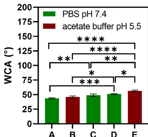
Fig. 7 WCA of all FS membrane formulations in PBS (pH 7.4) and acetate buffer (pH 5.5): (A) (HTCC/ALG/HTCC/FITC-BSA) 100 , (B) (HTCC/ALG) 200 , (C) (HTCC/ALG) 200 /HTCC/FITC-BSA, (D) (HTCC/ALG) 200 , and (E) (CHT/ALG) 200 . Data are presented as mean \pm SD of three independent experiments ( n = 3 , per condition) performed in triplicates. Significant differences were found for **** p \leq 0.0001 , *** p \leq 0.001 , ** p \leq 0.01 , and * p \leq 0.05 .
