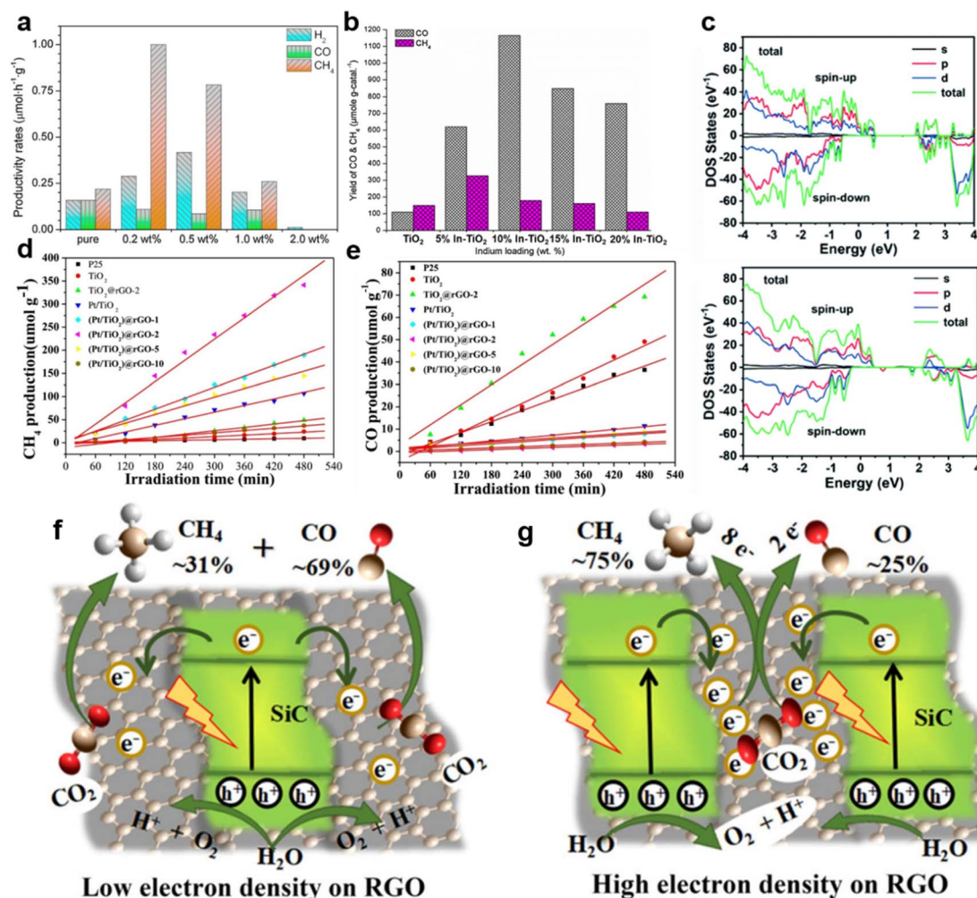
Fig. 5 (a) The production rates of pure \text{TiO}_2 and Mg-TiO 2 containing different amounts of Mg doping, reproduced with permission from ref. 100 copyright 2014 Elsevier. (b) The yield of products of In-TiO 2 with different amounts of In doping, reproduced with permission from ref. 101 copyright 2013 Elsevier. (c) Calculated total DOS (PDOS) and partial DOS (PDOS) plots of HC-NiCo-LDH without (upper) and with (lower) oxygen vacancies and Ni vacancies. Reproduced with permission from ref. 102 copyright 2018 Royal Society of Chemistry. (d) \text{CH}_4 production and (e) \text{CO} production over \text{TiO}_2 , \text{Pt/TiO}_2 , \text{TiO}_2 @rGO-2 and (\text{Pt/TiO}_2) @rGO- n catalysts. Reproduced with permission from ref. 56 copyright 2018 Elsevier. A schematic illustration of the electron density-dependent \text{CH}_4 selective production over SiC/rGO heterojunctions with (f) low electron density and (g) high electron density on rGO. Reproduced with permission from ref. 103 copyright 2018 Wiley.
