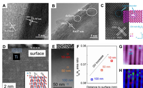
Fig. 2 HRTEM images of (A) pristine \text{SnS}_2 and (B) \text{SnS}_2 featuring Al doping 43 copyright © 2021 Elsevier B.V. (C) HAADF-STEM images of \text{V}_\text{O} -rich- \text{Bi}_2\text{O}_3 nanosheets, the scale bar is 2 nm. 45 Copyright © 2019, Springer Nature Limited. STEM image of cross-sectional \text{TiO}_2(110) single crystal (D) and large region (E). (F) Concentration of O vacancies increased from inner to surface regions. (G) STM image of the \text{TiO}_2 surface in the empty state. (H) STM image of the same region of (G), but in the filled state 46 copyright © 2018 American Chemical Society.
