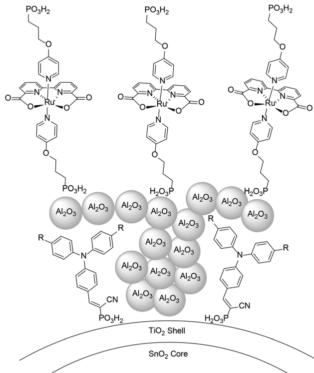
Fig. 22 4.5 nm \text{SnO}_2/\text{TiO}_2 particles sensitized with a triphenylamine photosensitizer, embedding a 7–10 Å \text{Al}_2\text{O}_3 protecting layer, exploited to anchor a Ru(bda) WOC. Reprinted from ref. 127 with permission from the American Chemical Society, copyright 2017.
