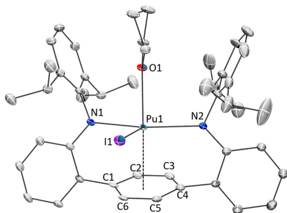
Fig. 3 ORTEP rendering of the solid-state molecular structures of 3^{Pu} \cdot \text{THF}_{0.66} \text{Et}_2\text{O}_{0.33} . Hydrogen atoms and co-crystallized solvents are removed for clarity. Ellipsoids are shown at the 50% probability level. Complexes 3^{Ce} , 3^U and 3^{Np} are structurally analogous and can be found in the ESI for this document (S5–S7†).
