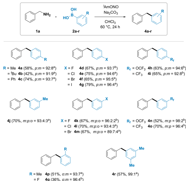
Fig. 3 Arylboronic acid scope of the deaminative coupling between benzylamines and arylboronic acids. Reaction conditions: benzylamine ( 1a , 2.0 mmol), arylboronic acid ( 2a–r , 0.5 mmol), isoamyl nitrite (2.5 mmol), sodium carbonate (0.5 mmol), chloroform (1.25 mL), 60 °C, 24 h. Isolated yields after flash column chromatography. a Isomer ratio determined by 13 C NMR. b Isomer ratio determined by 19 F NMR.
