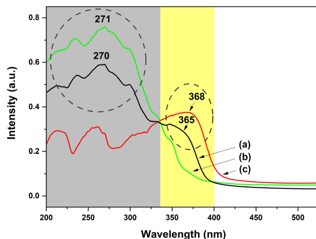
Fig. 11 UV-vis absorption spectra of the PS-Eu 1 -Tb 60 fiber membrane (a), the PS-Tb fiber membrane (b) and the PS-Eu fiber membrane (c).
