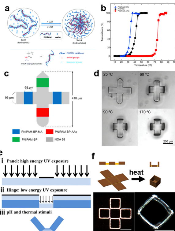
Fig. 12 (a) Schematic illustration of thermos-responsive LCST behavior of PNIPAM. Reproduced with permission. 321 Copyrights 2020, Royal Society of Chemistry. (b) Temperature dependence of transmittance at 515 nm of PNIPAM copolymer solutions in ionic liquid at a heating rate of 1 °C min -1 . (c) Schematic illustration of the design for a sequential self-folding PNIPAM-based hydrogel sheet in the plan view (d) Optical images of a self-folding micropatterned PNIPAM-based hydrogel sheet in ionic liquid at different temperatures throughout heating. Reproduced with permission. 325 Copyright 2017, American Chemical Society. (e) Schematic of P(NIPAM-AAc) hydrogel strip with (i) thick, fully crosslinked panel and (ii) thin, gradient crosslinked hinge. (iii) Schematic deformation of hydrogel strip under Ph and thermal stimuli (f) Schematic and optical images of temperature responsive self-folding. Reproduced with permission. 327 Copyright 2014, IOP Publishing.
