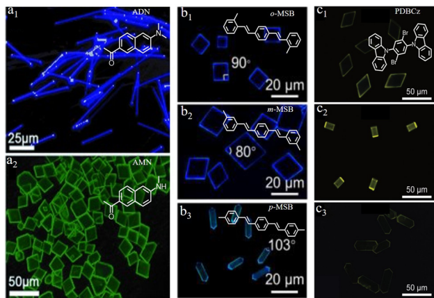
Fig. 3 Tunable microstructures of organic crystals. (a) The PL microscopy images of 1D and 2D nanostructures based on naphthalene derivatives with different amino groups. 54 Copyright 2013 Wiley-VCH Verlag GmbH & Co. KGaA, Weinheim. (b) The PL microscopy images of o -MSB, m -MSB, and p -MSB microsheets with different side chains. 55 Copyright 2022 Elsevier. (c) The PL microscopy images of concentration dependent PDBCz microsheets. Insets are the corresponding molecular formulas. 60 Copyright 2021 The Royal Society of Chemistry.
