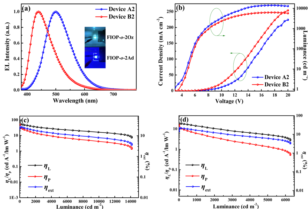
Fig. 7 (a) EL spectra of device A2 and device B2 . (b) Current density–voltage–luminance ( J–V–L ) characteristics for the optimized devices. Relationship between EL efficiencies and luminance of (c) device A2 , and (d) device B2 .
