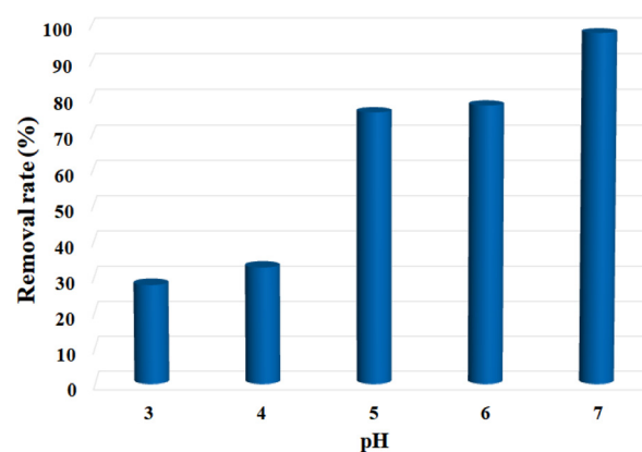
Fig. 3 pH effect on the removal efficiency of Pb 2+ by MOF nanosheets. C_0 = 10 ppm, m_{\text{adsorbent}} = 5 mg, V = 50 mL, pH = 3.0–7.0.
