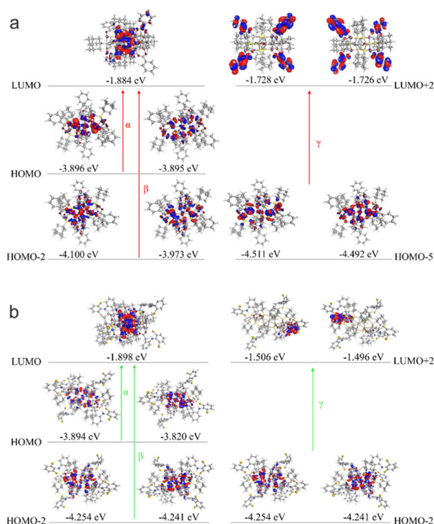
Fig. 4 Orbitals involved in the \alpha , \beta and \gamma transitions of \text{Cu}_{14}\text{-1} (a) and \text{Cu}_{14}\text{-2} (b).
