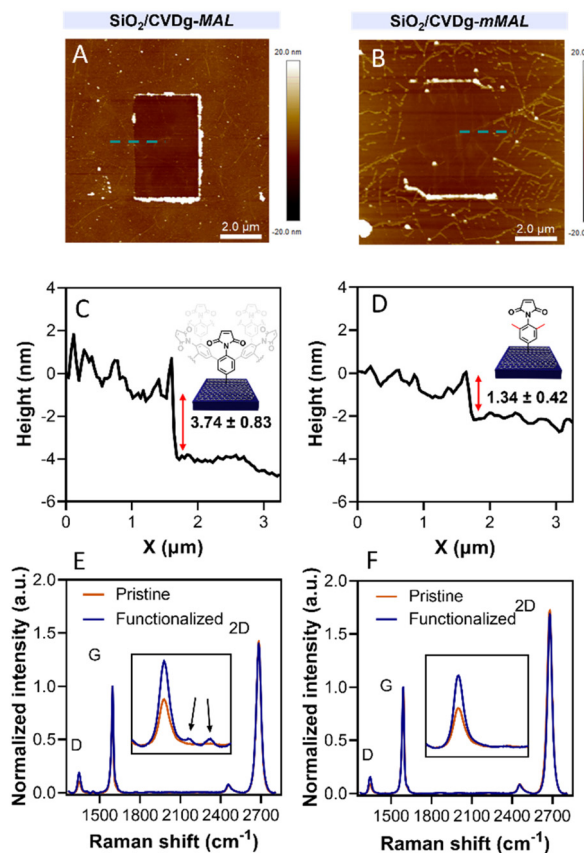
Fig. 3 (A and B) AFM scratching images and (C and D) height profiles of SiO 2 /CVDg-MAL (A and C) and SiO 2 /CVDg-mMAL (B and D). (E and F) Raman spectra of SiO 2 /CVDg-MAL (E) and SiO 2 /CVDg-mMAL (F) before and after the reaction.
