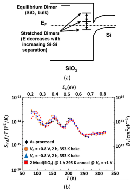
Fig. 7 (a) Schematic diagram of dimer (unrelaxed) O vacancy energy levels in bulk and near-interfacial \text{SiO}_2 . Band narrowing and near-interfacial strain reduce O vacancy energies, facilitating electron capture. Electron capture relieves strain, increasing the energy, and favoring emission. Reproduced from ref. 107 with permission. Copyright 107 Institute of Electrical and Electronics Engineers. (b) Normalized 1/f noise (left y-axis) and effective border-trap density from eqn (15) (right y-axis) vs. temperature for nMOS transistors with \text{SiO}_2/\text{HfO}_2 gate dielectrics before and after bias-temperature stress at 353 K and 10 keV X-ray irradiation to 2 Mrad( \text{SiO}_2 ). The energy scale on the upper x-axis is from eqn (7). Reproduced from ref. 154 with permission. Copyright 2023 Institute of Electrical and Electronics Engineers.
