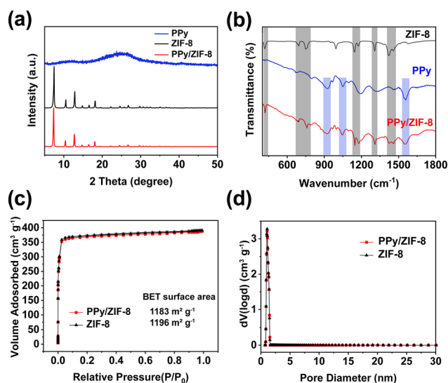
Fig. 2 Structural characterization. (a) Powder XRD patterns and (b) FTIR spectra of PPY NPs, ZIF-8, and PPY/ZIF-8. (c) \text{N}_2 adsorption-desorption isotherms and (d) pore size distributions of ZIF-8 and PPY/ZIF-8 based on the NLDFT method.
