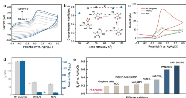
Fig. 2 Electrocatalytic oxidation of AA. (a) CVs of Rh SAzymes in 10 mM AA and 0.1 M PBS at different scan rates (20, 40, 60, 80, 100, and 120 \text{mV s}^{-1} ) and (b) the corresponding \beta versus scan rate. (c) Background-corrected CV curves of Rh SAzymes, RhO x /C, and Rh/C at a scan rate of 50 \text{mV s}^{-1} in 10 mM AA and 0.1 M PBS. (d) The corresponding peak currents and mass activities of Rh SAzymes, RhO x /C, and Rh/C for AA oxidation. (e) Comparison of the anodic peak potential for Rh SAzymes and previously reported catalysts. 42–50
