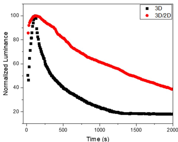
Fig. 6 Operational stability of the 3D/2D perovskite-based device and related reference device (3D).
