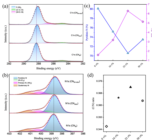
Fig. 4 XPS CN analysis. High-resolution (a) C 1s and (b) N 1s XPS spectra of CN_M , CN_{M+mlm} , and CN_{M+mlm} . (c) Calculated percentage of pyridinic N and free NH_2 species for various amounts of EG (v%) used in the hydrothermal treatment during CN_{M+mlm} syntheses, calculated from N 1s spectra. (d) Atomic C/N ratio obtained from survey scans of CN_{M+mlm} prepared with varying EG content. The experimental points in (a) and (b) are fitted with a red line, which is deconvoluted into peaks corresponding to the indicated chemical species. The lines connecting the diamonds and triangles in (c) serve as a guide to the eye.
