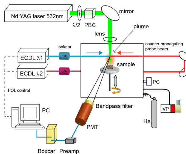
Fig. 1 Experimental setup for doppler-free ablation fluorescence spectroscopy. PMT: photomultiplier, PBC: polarization beam splitter, ECDL: external cavity diode laser, FOL: fringe offset locking, PG: Pirani gauge, and VP: vacuum pump.
