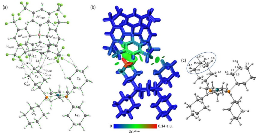
Fig. 8 (a) QTAIM molecular graph with Eq-2 in [1\text{-propane}][\text{BAR}^{\text{F}}_4] with BCPs in green and showing selected atoms and BCP electron densities (a.u. \times 10^{-3} ). Bond paths with \rho(r) < 0.001 a.u., intramolecular bond paths and ring critical points (RCP) are omitted for clarity. (b) IGMH plot where the cation and anion are defined as separate fragments. \text{Sign}(\lambda_2)\rho -coloured isosurfaces are plotted with \delta G^{\text{inter}} = 0.003 a.u. and atoms are coloured by \delta G^{\text{atom}} . (c) \% \delta G^{\text{atom}} contributions on the cation that are above 1%, with the propylene motif highlighted (see text for details).
