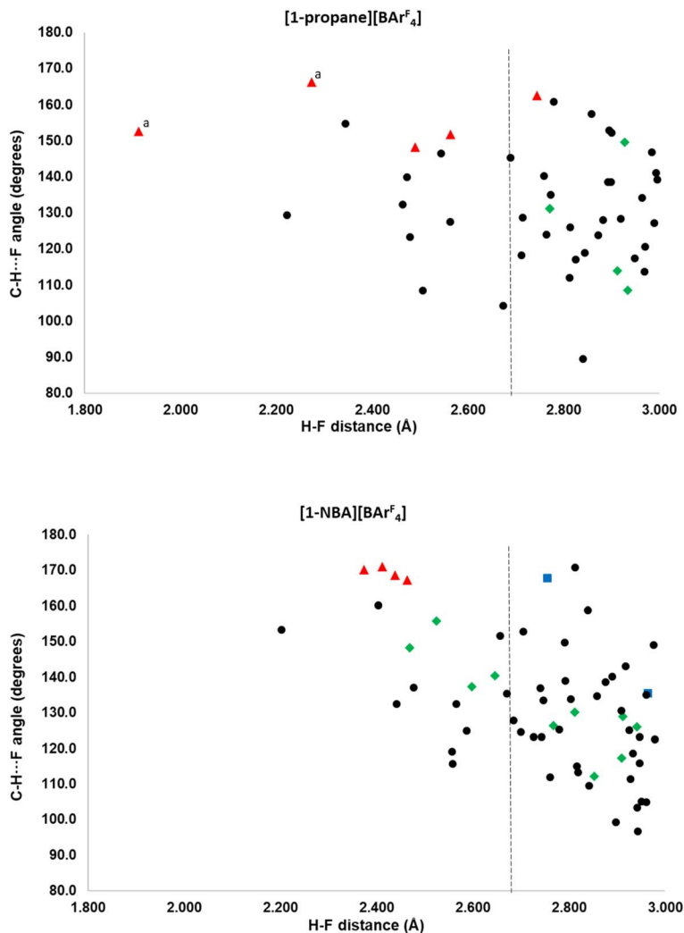
Fig. 4 Scatterplots of H \cdots F distance (Å) vs. C–H \cdots F angle (degrees) for the [1-NBA] ^+ and [1-propane] ^+ cations within the octahedral arrays of neighbouring [BAr _4 ] ^- anions. The dashed vertical line indicates the sum of the van der Waals radii for H and F. a Data points correspond to two equivalent H \cdots F contacts.
