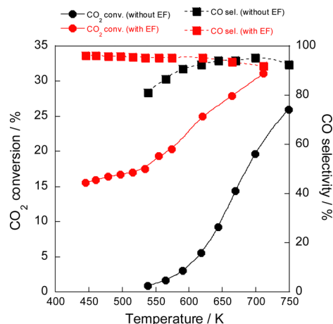
Fig. 1 Temperature dependence of CO 2 conversion and CO selectivity in the RWGS reaction with/without the electric field (EF) over the Ru(col)/ZrTiO 4 catalyst; CO 2 :H 2 :Ar = 1:1:2; 100 SCCM total flow rate; 100 mg catalyst weight; 0 or 5.0 mA imposed current.
