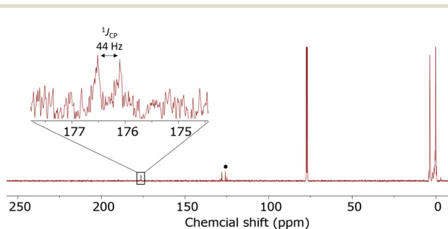
Fig. 8 ^{13}\text{C}\{^1\text{H}\} NMR spectra for the reaction of (\text{Me}_3\text{Si})_3\text{P}_7 with \text{CO}_2 . Dissolved \text{CO}_2 marked with •.
