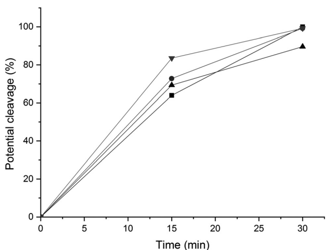
Fig. 11 Potential conversion of the \beta -O-4'( \beta ) (—■—), \beta -O-4'( \alpha ) (—●—) and \beta -5' (—▲—) and 5-5' (—▼—) environments according to the HMBC spectra with the integration of the signals at (4.19, 146.77 ppm), (4.97, 108.42 ppm), (5.08, 110.29 ppm) and (6.89, 124.09 ppm) respectively.
