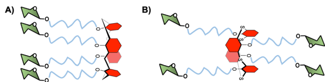
Fig. 4 (A) Cone conformation of the glycolix[4]arenes, and (B) 1,3-alternate conformation of glycolthiacalix[4]arenes.
