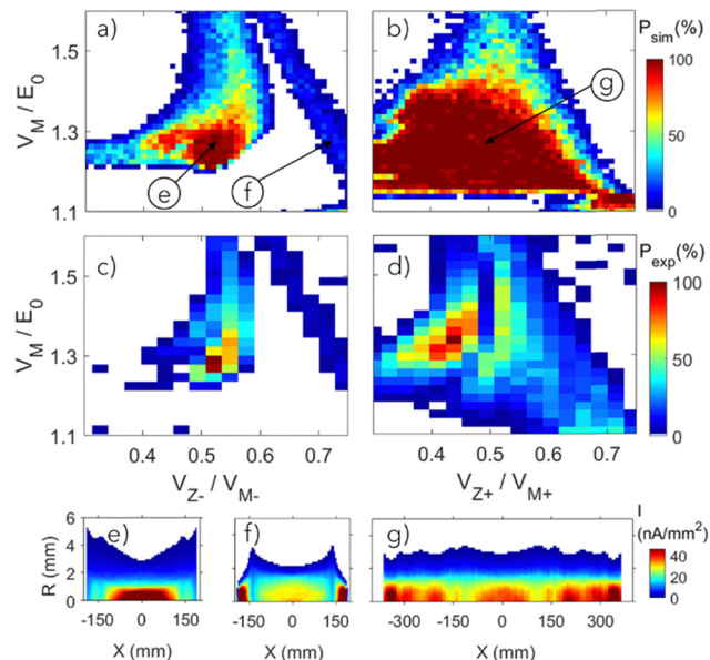
Fig. 2 Two dimensional scan of the voltages applied to the main mirror electrode ( V_M ) and the Einzel lens ( V_Z ) with color coded Trapping efficiencies, P_{sim} for simulated data and relative experimental efficiencies P_{exp} . Figures a and b present SIMION simulation for the HEIBT inner (a) and outer (b) HEIBT traps, while figures c and d show the normalized experimental results. (e)–(g) present the simulated ion current densities ( I ) along the trap for selected V_M and V_Z potentials.
