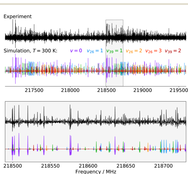
Fig. 5 Portions of the spectrum of p -CEB recorded in this work using the source-frequency modulation millimeter-wave spectrometer and comparison with simulations (at 300 K) of the pure rotational spectrum of the molecule in the six vibrational states assigned in this study (from \nu = 0 to \nu_{39} = 2 by increasing energy, see Fig. 2). The second derivative of the simulation is plotted, for better comparison with the experimental spectrum. The lower panel is a zoom-in on the region highlighted in gray in the upper panel.
