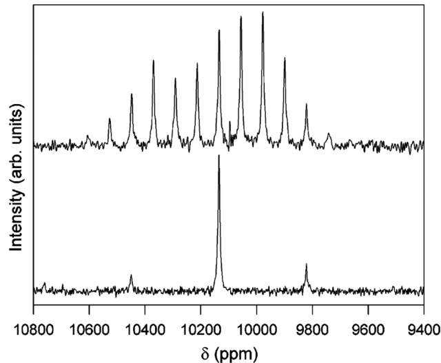
Fig. 12 ^1\text{H} - ^{103}\text{Rh} CP-MAS NMR spectra of [[(\text{H}_2\text{O})_4\text{Rh}(\mu_2\text{-OH})_2\text{Rh}(\text{H}_2\text{O})_4]_n(\text{dmtos})_n] \cdot 8\text{H}_2\text{O} comparing spinning rates of 1.0 (top) and 4.0 kHz (bottom). Both spectra acquired with 8 ms contact time, 5 s relaxation delay for 12 000 (top) and 15 800 (bottom) acquisitions. 37 Reproduced from the ref. 37 with permission from the American Chemical Society, copyright 2006.
