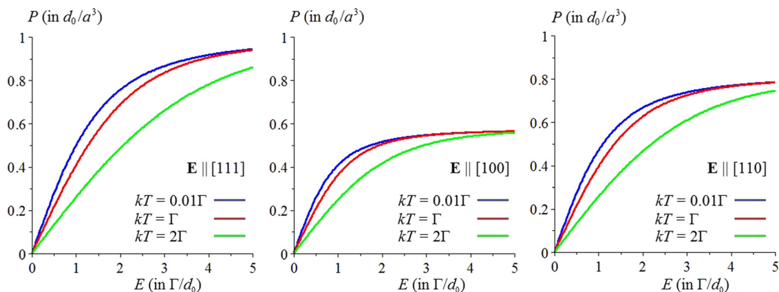
Fig. 6 Variation of the polarization P (in units of d_0/a^3 ) of the cluster [\text{BO}_6] with the external electric field E (in units of \Gamma/d_0 ) along the main symmetry axes [111], [100] and [110] at three temperatures. Reprinted from ref. 40. Copyright 2017 IOP.
