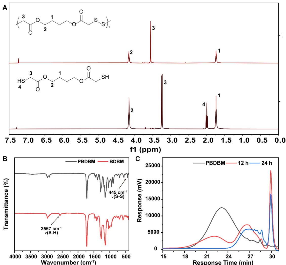
Fig. 1 Characterization of poly(disulfide)s (PBDBM). (A) ^1\text{H} NMR spectra of PBDBM and BDBM. (B) FT-IR spectra of PBDBM and BDBM. (C) GPC profiles of PBDBM and PBDBM after incubation with dithiothreitol for 12 and 24 h.
