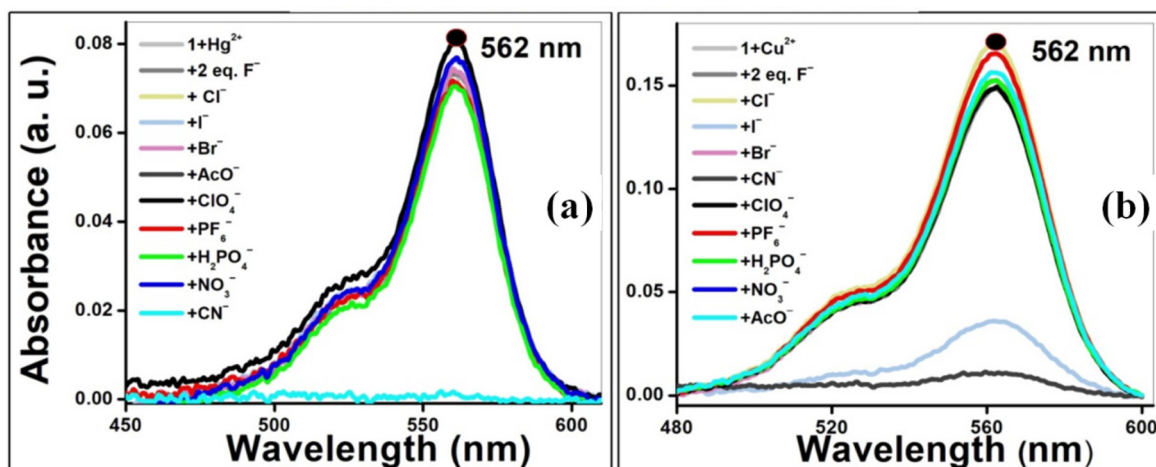
Fig. 5 (a) UV-visible spectra of 1 + \text{Hg}^{2+} ([ 1 ] = 10 \mu\text{M} , 1 : \text{Hg}^{2+} = 1 : 1) with different anions in acetonitrile–water (1 : 1) medium. (b) UV-visible spectra of 1 + \text{Cu}^{2+} ([ 1 ] = 10 \mu\text{M} , 1 : \text{Cu}^{2+} = 1 : 1) with different anions in acetonitrile–water (1 : 1) medium.
