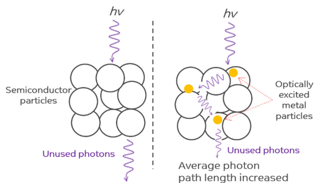
Fig. 5 Photon scattering mechanism. Adapted from ref. 99.
