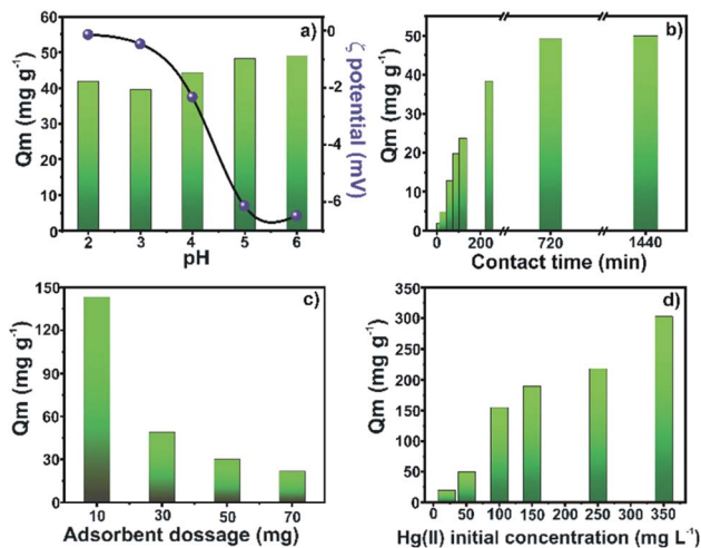
Fig. 4 Effect of (a) pH; (b) contact time; (c) adsorbent dosage; (d) Hg(II) concentration on the adsorption capacity of Zr-MOF@Fe 3 O 4 . Conditions: mass of Zr-MOF@Fe 3 O 4 = 30 mg, [Hg(II)] = 50 \text{mg L}^{-1} , volume = 30 mL, time = 12 h (change accordingly).
