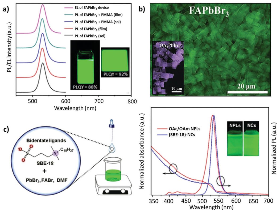
Fig. 8 (a) PL spectra for the colloidal 2D \text{FAPbBr}_3 perovskite and its composite with PMMA, where the inset depicts the 2D \text{FAPbBr}_3 perovskite colloidal solution (left) and spin-coated thin film (right) under UV excitation in toluene solution and thin films. (b) SEM image of \text{FAPbBr}_3 NPLs, where the inset depicts the SEM image of \text{OA}_2\text{PbBr}_4 . (c) Schematic illustration of the synthesis process of \text{FAPbBr}_3 NCs (left) and the PL absorption and emission spectra of (SBE-18)-capped \text{FAPbBr}_3 NCs and OA/OAM-capped \text{FAPbBr}_3 NPLs (right), with insets showing their colloidal solutions under 365 nm UV light. Panel (a) adapted from ref. 159. Copyright 2017 American Chemical Society. Panel (b) adapted from ref. 161. Copyright 2018 WILEY-VCH Verlag GmbH & Co. KGaA, Weinheim. Panel (c) reproduced with permission from ref. 162. Copyright 2019 American Chemical Society.
