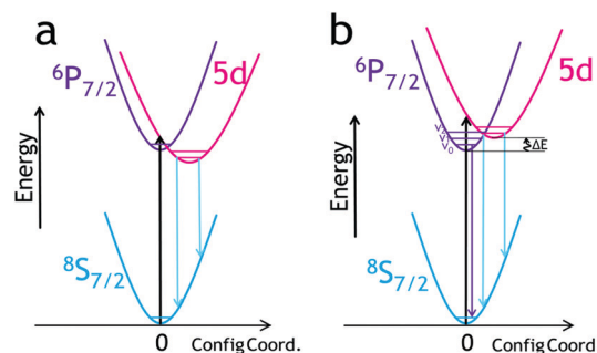
Fig. 1 Schematic diagram of the energy levels of the Eu 2+ ion. In (a), the 5d level is positioned below the 6 P 7/2 one, which precludes the 6 P 7/2 \rightarrow 8 S 7/2 radiative relaxation, and only the 5d \rightarrow 4f luminescence occurs. In (b), both narrow and broadbands corresponding to the 6 P 7/2 \rightarrow 8 S 7/2 and 5d \rightarrow 4f( 8 S 7/2 ) transitions, respectively, are possible, and their relative intensities (populations) are mainly governed by thermal coupling (situation valid for the SrB 4 O 7 :Eu 2+ system).
