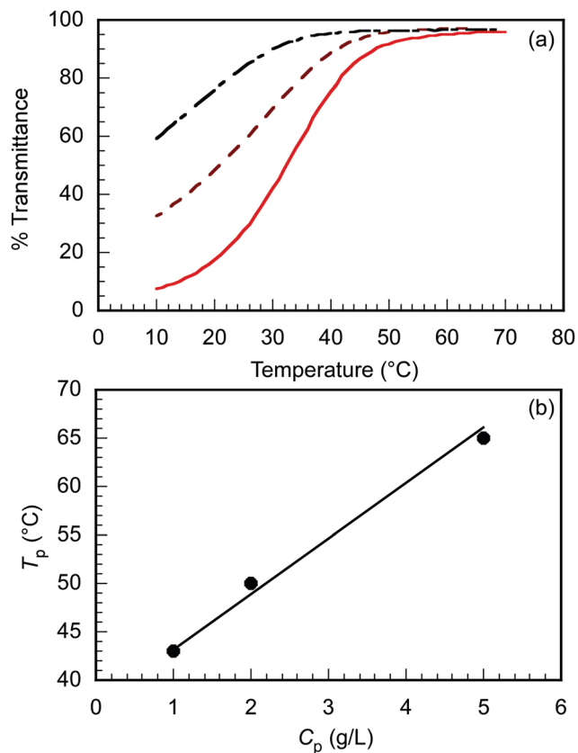
Fig. 2 (a) Percent transmittance (% T ) of EUM in PBS at various C_p = 1.0 (.....), 2.0 (---), and 5.0 \text{g L}^{-1} (—) as a function of temperature with the cooling process, and (b) phase transition temperature ( T_p ) of EUM in PBS as a function of C_p .
