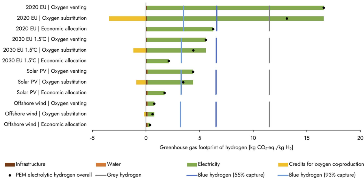
Fig. 2 The greenhouse gas footprint of PEM electrolytic hydrogen for different electricity sources and multi-functionality approaches in kg CO 2 -equivalents (kg CO 2 -eq. ) per kg H 2 . The benchmarks grey and blue hydrogen (the latter with a CO 2 capture rate of 55% or 93%) are based on Bauer et al. 7 and were harmonised for each electricity source. The 2020 EU electricity mix and the 2030 mix for a 1.5 °C-consistent emissions pathway are based on the integrated assessment model REMIND; 25 solar PV located in Europe was based on Bosmans et al. ; 14 offshore wind was based on Bonou et al. 26 Infrastructure emissions are based on 3000 full-load hours for the purely renewable sources while on 8000 full-load hours for the grid mixes. LCA inputs were based on Bareiß et al. 10 and background life-cycle inventory data on the Ecoinvent database version v3.7.1, using allocation at point of substitution. The ReCiPe2016 method (H) v1.05 was used at midpoint level to quantify the greenhouse gas footprints. Details on how we applied different methods to deal with multi-functionality can be found in the ESI.† The contribution of oxygen is shown as having a negative greenhouse gas footprint because it is a prevented emission; it does not signify carbon dioxide removal.
