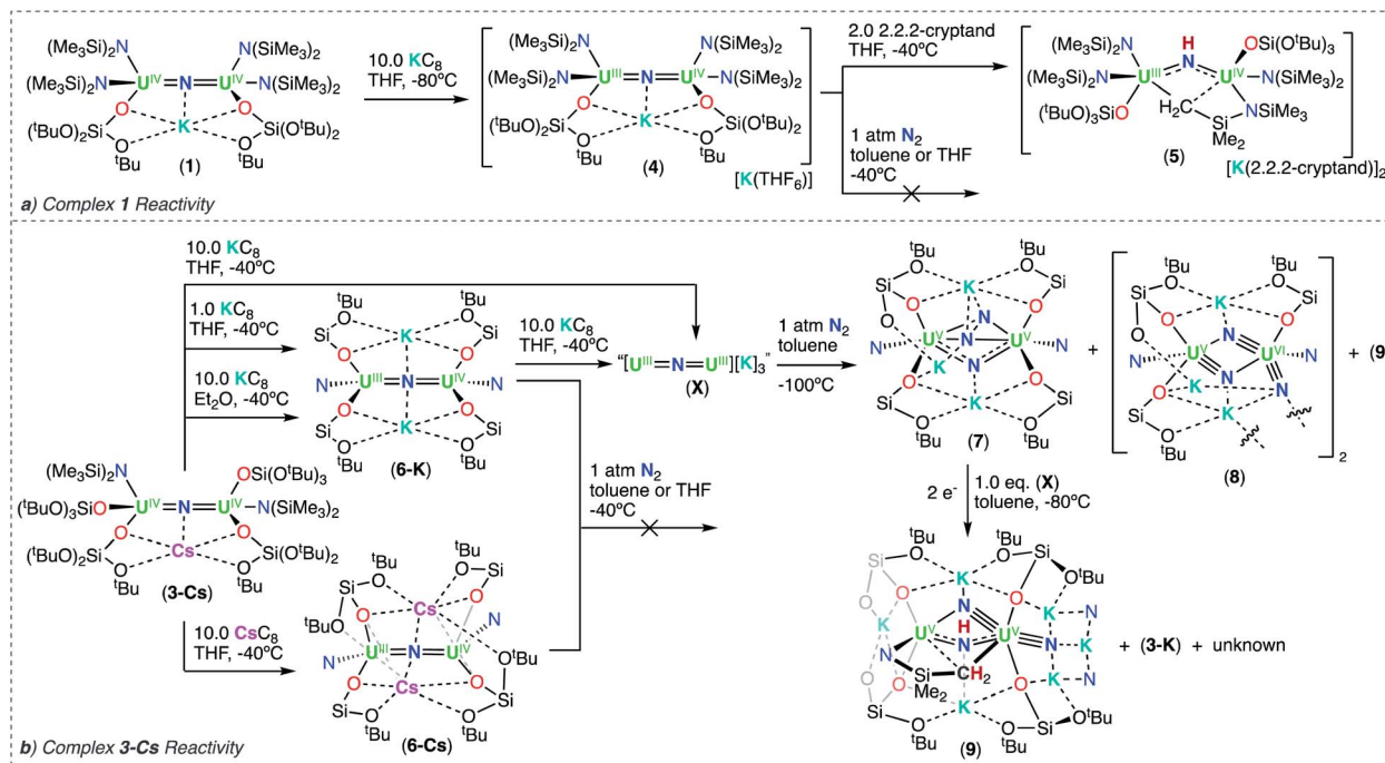
Scheme 3 Reactivity of complexes (a) 1 and 4 and (b) 3-Cs, 6-K, 6-Cs, X, and 7. The -\text{O}^t\text{Bu} and -(\text{SiMe}_3)_2 substituents on complexes 6-K, 6-Cs, 7, 8, and 9 were omitted for clarity.
