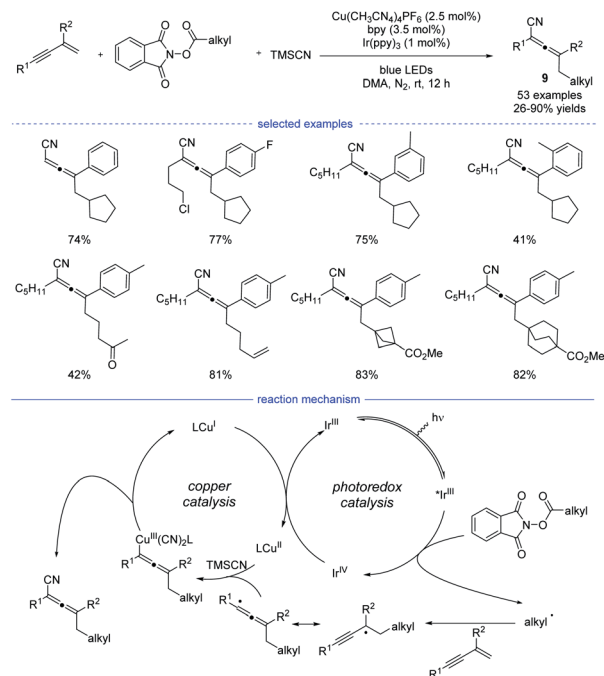
Scheme 6 Cu-catalyzed regioselective 1,4-carbocyanation of 1,3-enynes with redox-active esters.
