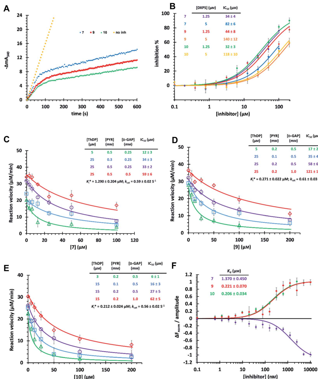
Fig. 4 (A) Time-dependent progress curves of the final hits. Conditions can be found in ESI Methods 3.2.7.† (B) Dose–response curves of the final hits by varying Mt DXPS concentration. (C), (D) and (E) Mode-of-inhibition study and determination of K_i^* of compounds 7, 9 and 10, respectively. Color code: reference condition: purple; varying [ThDP]: green; varying [PYR]: blue; varying [D-GAP]: red. (B)–(E) The reaction velocity was measured after 200 s, when the slow-onset phase was considered complete. (F) Determination of K_D of the final hits with microscale thermophoresis (MST) (binding curves). Curve shape is dependent on molecular movement during measurement and has no influence on K_D determination.
