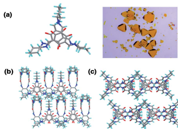
Fig. 2 (a) SCXRD and crystal image of OC1 . (b) OC1 self-assembled through hydrogen bonding interactions. (c) Packing of OC1 along b -axis.
