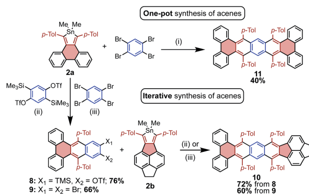
Scheme 4 Synthesis of acenes via the multiple addition of stannoles to benzynes. Reagents and conditions: (i) aryne (0.5 equiv.), ^n\text{BuLi} (1.1 equiv.), toluene, 23 °C; (ii) aryne (1.1 equiv.), [\text{nBu}_4\text{N}][\text{Ph}_3\text{SiF}_2] (3 equiv.), DMAD (1.5 equiv.), toluene, 60 °C; (iii) aryne (2 equiv.), ^n\text{BuLi} (1.1 equiv.), toluene, 23 °C.
