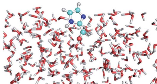
Fig. 3 Snapshot from the QM/MM MD simulation of IC ( S_0 ) at the air–water interface.
