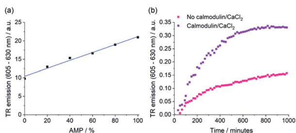
Fig. 7 Real-time monitoring of phosphodiesterase (PDE) activity. (a) Simulation of the PDE reaction, recording the time-resolved emission of [\text{Eu} \cdot \text{mBOH}_2]^+ with increasing % AMP. Conditions: 100 \mu\text{M} cAMP + AMP, 5 mM \text{MgCl}_2 , 5 \mu\text{M} [\text{Eu} \cdot \text{mBOH}_2]^+ , 10 mM HEPES at pH 7.0. (b) Real-time monitoring of the PDE-catalysed conversion of cAMP to AMP using the time-resolved emission of [\text{Eu} \cdot \text{mBOH}_2]^+ , comparing the change in rate of reaction upon activation with calmodulin (2 \mu\text{M} ) and \text{CaCl}_2 (60 \mu\text{M} ). Conditions: 200 \mu\text{M} cAMP, 4 \mu\text{L} PDE (0.1 \text{mg mL}^{-1} ), 5 mM \text{MgCl}_2 , 10 \mu\text{M} [\text{Eu} \cdot \text{mBOH}_2]^+ , 10 mM HEPES at pH 7.0, \lambda_{\text{exc}} = 292\text{--}366 nm, \lambda_{\text{em}} = 615\text{--}625 nm, integration time = 60–400 \mu\text{s} .
