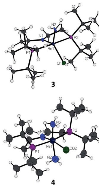
Fig. 1 Solid-state structures of \text{Re} –amide complex 3 and \text{Re}(\text{NH}_3)_2 complex 4 ( \text{BAR}_4^{\text{F}} ion omitted) with thermal ellipsoids at 50% probability.
