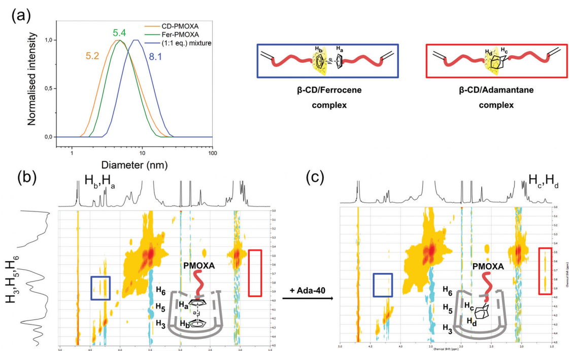
Fig. 3 (a) Size distribution of CD-PMOXA, Fer-PMOXA and their 1 : 1 molar mixture in at 25\text{ }^\circ\text{C} ( c = 1\text{ g mL}^{-1} ). (b) 2D NOESY spectrum of 1 : 1 molar mixture of CD-PMOXA and Fer-PMOXA ( 5\text{ mmol L}^{-1} ) in \text{D}_2\text{O} at 30\text{ }^\circ\text{C} and (c) 2D NOESY spectrum after the addition of Ada-40 (Adamantane-PMOXA).
